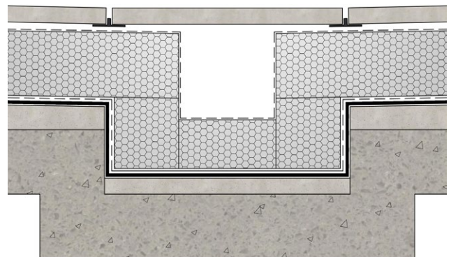
Figure 7. Ballasted inverted roof - insulation over internal gutter
