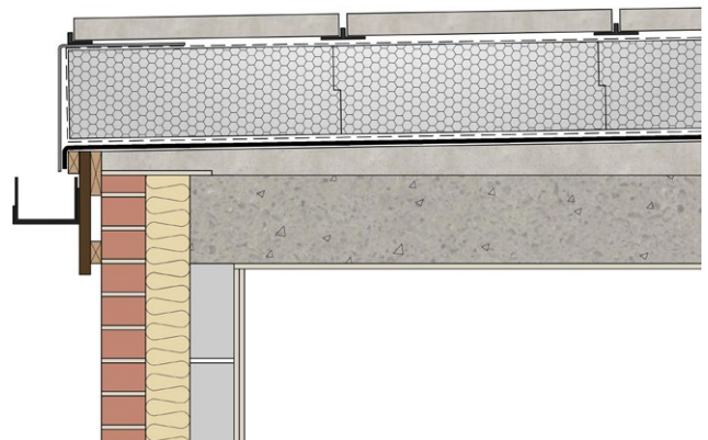
Figure 8. Ballasted inverted roof – detail at eaves
