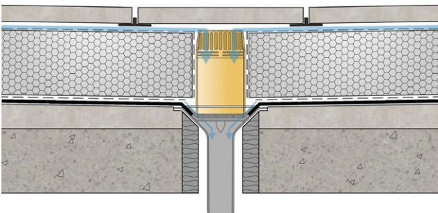
Figure 6. Ballasted inverted roof – outlet protected by paving slabs
