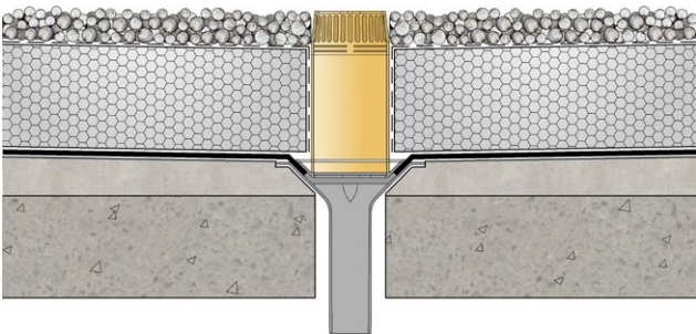
Figure 5. Ravatherm XPS X MK system in the inverted roof
