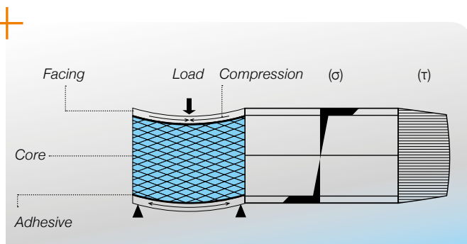
21 Shear forces resulting from loading of the composite panel
